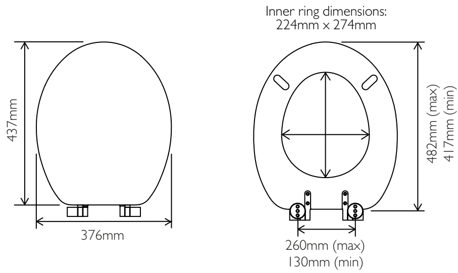
General seat dimensions Max/min fixing adjustment
