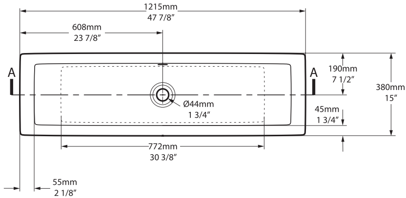
Top view
