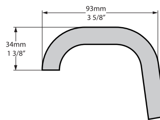
Rim detail
